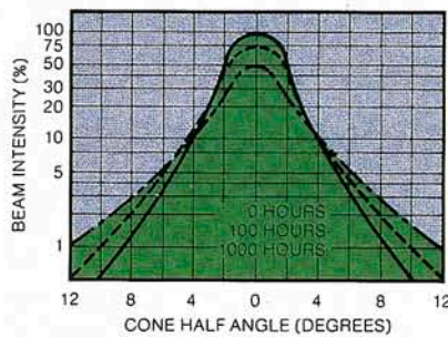
Figure 3: TYPICAL BEAM PROFILES
